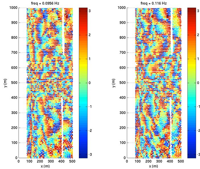
Figure 3. Phase maps for the entire collection domain for 2 of 11 possible frequencies from an example analysis. Colors show wave phase varying reasonably from -\pi to \pi with scales typical of ocean waves, confirming that the input stack data appears to have useful signals.
