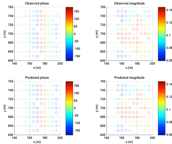
Figure 4. Phase maps of the dominant EOF within an example analysis tile with EOF phase on the left and magnitude of the right. The observed values (upper panel) should match the modeled values (lower panel). This example is MATLAB window 4, so corresponded to the fourth-most important analysis frequency for this tile.
